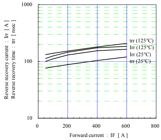
Reverse recovery characteristics (typ.) Vcc=300V, VGE=±15V, Rg=6.8Ω
