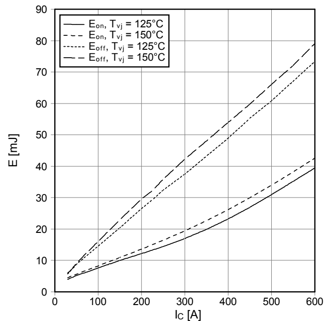
Schaltverluste IGBT-Wechselr. (typisch) switching losses IGBT-inverter (typical) E_{on} = f(I_c), E_{off} = f(I_c) V_{GE} = \pm 15\text{ V}, R_{Gon} = 1.3\ \Omega, R_{Goff} = 1.3\ \Omega, V_{CE} = 600\text{ V}
